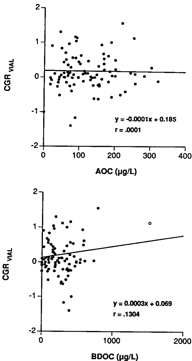
Figure 6 Correlations of : (A) CGR and AOC concentrations ; and (B) CGR and BDOC concentrations. Open symbols are data excluded from the correlations.
