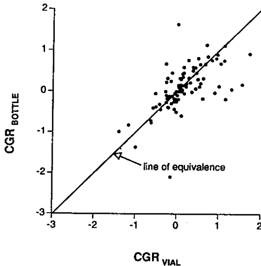
Figure 3 Influence of incubation vessel on CGR values.
